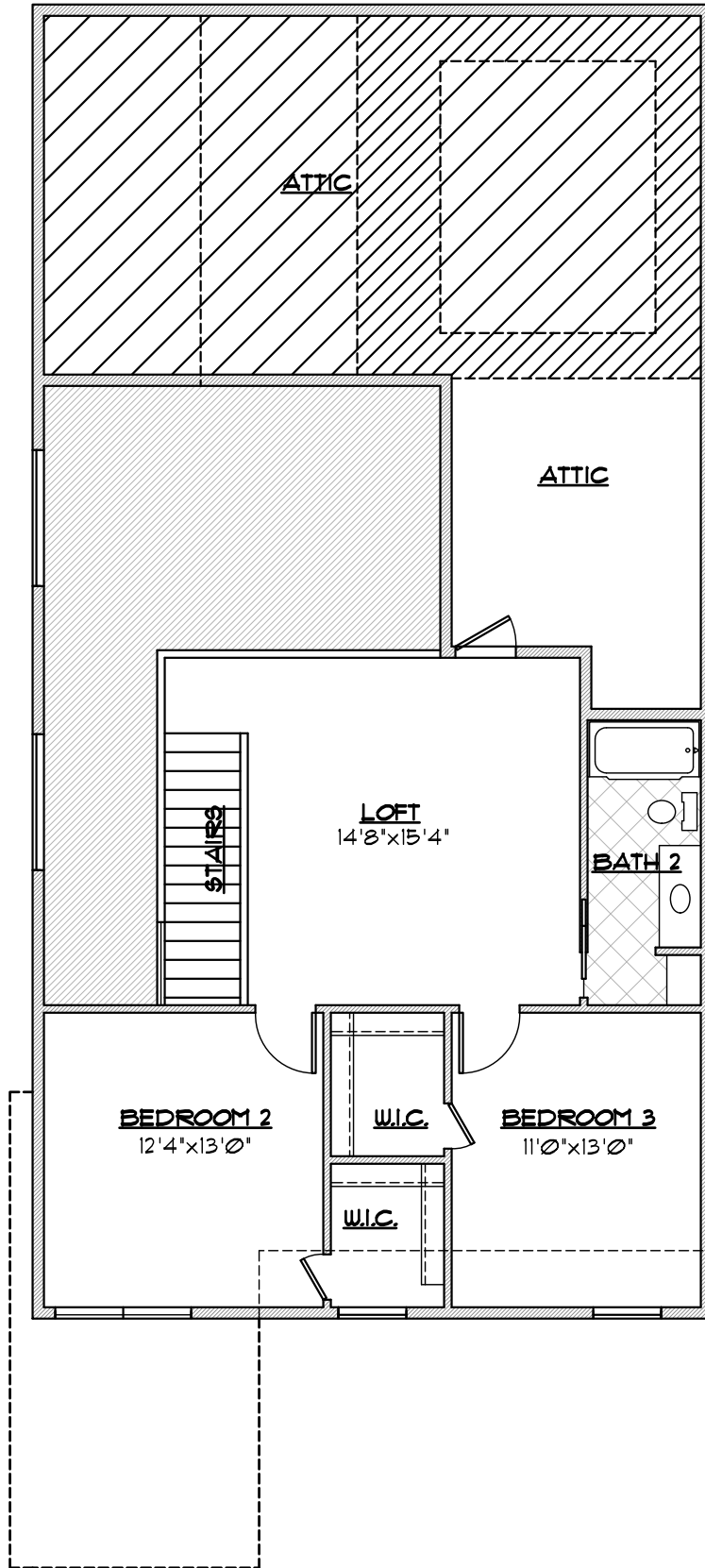
SECOND FLOOR PLAN 1/8" = 1'0"
